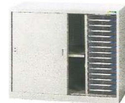
06009 A4鐵拉門邊15小抽 J-A4-O15S-US W900xD450xH740(mm)
