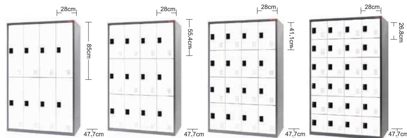
FC-408 密碼鎖 (14-02) FC-408K一般鎖 (14-05) 1182W x 510D x 1800H mm
